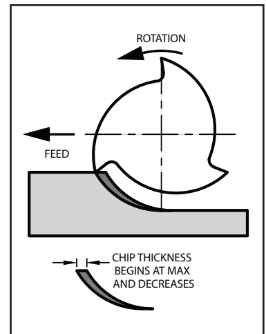
Figure 3: Climb Milling
