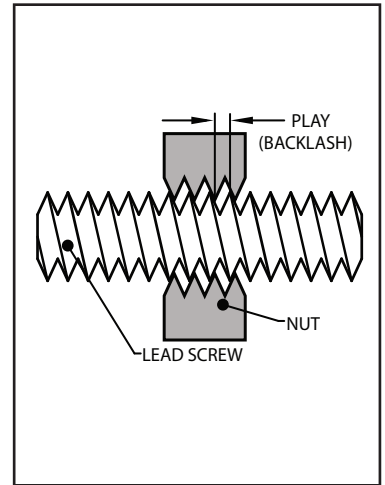
Figure 1: Backlash
