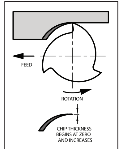
Figure 2: Conventional Milling
